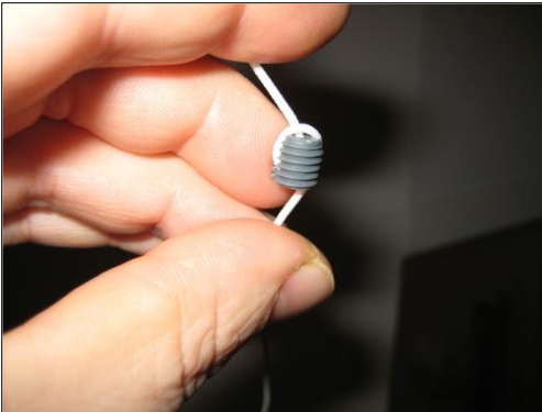
Thread the cord in a loop around the locking screw, making sure the cord is well placed in the grooves
