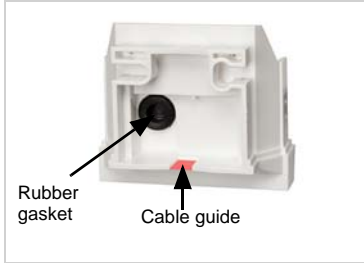
Fig. 11 Break the cable guide off.
