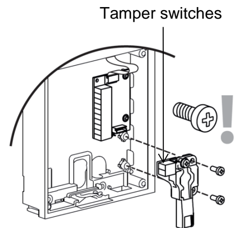
Figure 2. Tamper switch installation
