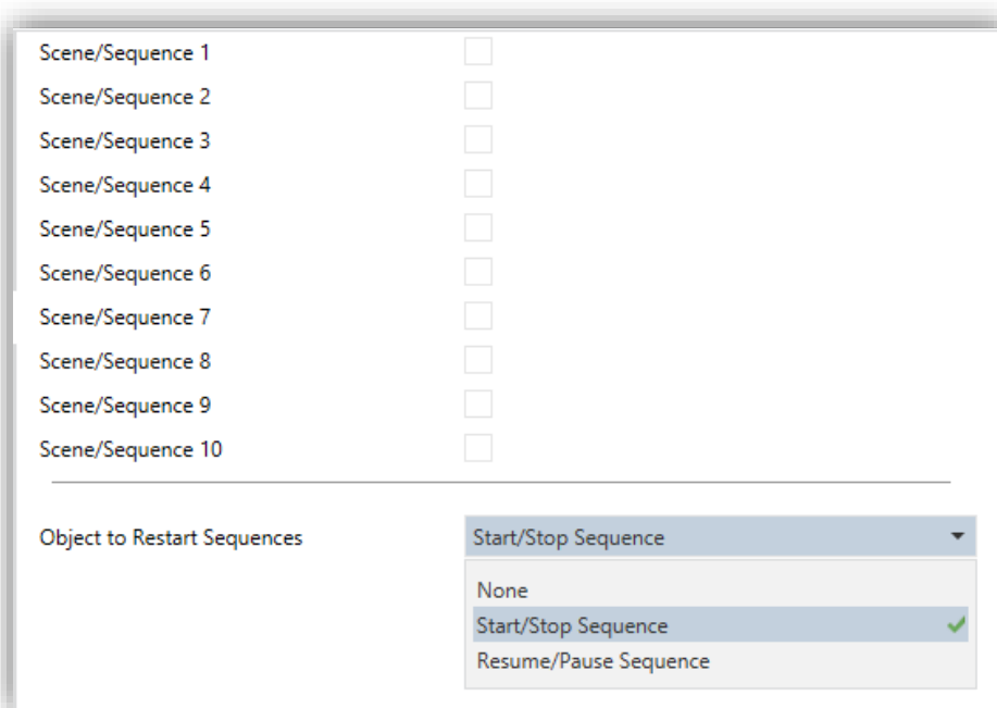
Figure 17 Scenes/Sequences.
