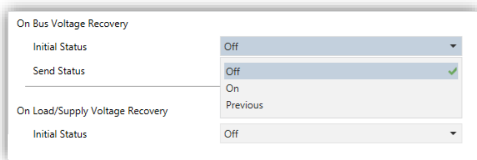
Figure 23 Initialisation Settings.
