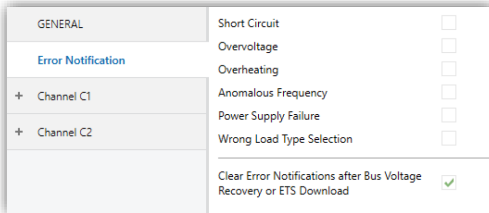
Figure 24 Error Notification.
