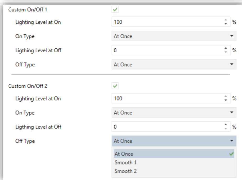
Figure 14 Custom On/Off.
