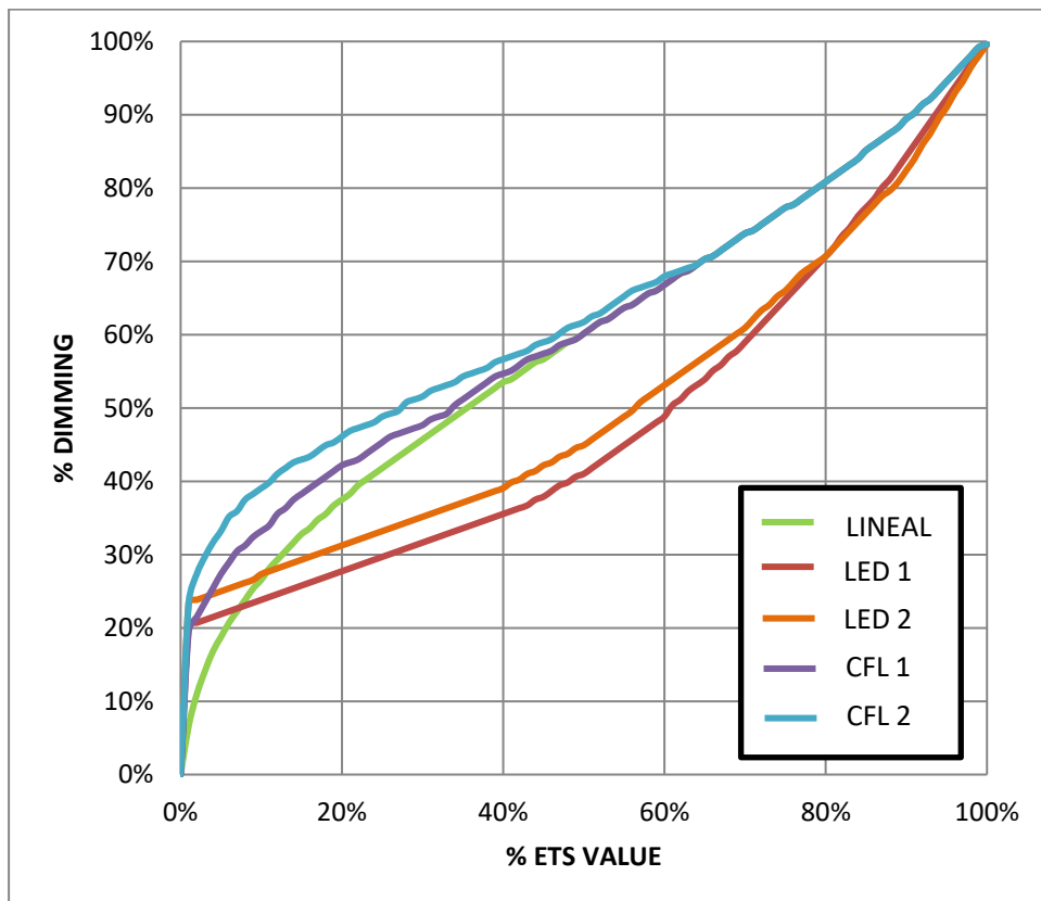
Figure 10 Dimming Patterns for LED and CFL loads.
