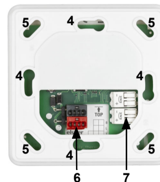
Fig. 2: Back view with mounting 4/5 Screw holes for different sockets. Fastening with 2 screws is sufficient. For wall mounting, use a fixing material suitable for the ground! 6 KNX bus terminal +/- for connection when mounted on a socket 7 Spring-loaded terminals KNX bus for mounting directly on the wall
