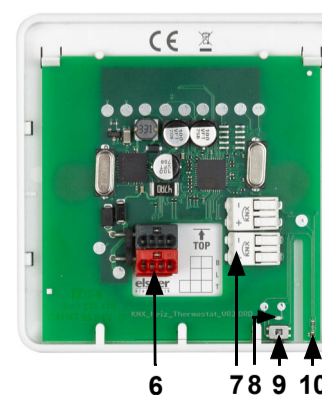
Fig. 3: Back view without mounting 6 KNX bus terminal +/- for connection when mounted on a socket 7 Spring-loaded terminals KNX bus for mounting directly on the wall 8 Programming LED 9 Programming button (recessed) for teaching device 10 Temperature sensor
