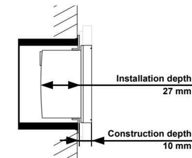
Fig. 2: Sectional drawing. The Cala KNX T 201/202 Sunblind push button fits in a standard connector socket (Ø 60 mm, depth 42 mm). The frame is not included in the delivery!
