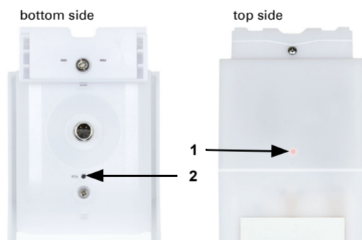
Fig. 18 1 Programming LED (under the semi-transparent lid) 2 Programming button for teaching the device
