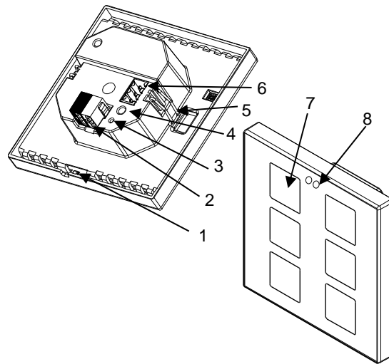
Figure 1 Schematic diagram.
